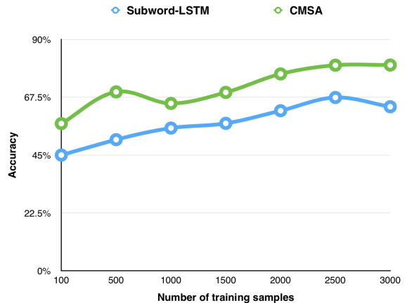
Figure 4: Performance on varying training data size
